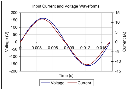
Input AC Current Waveform (ITHD = 6.04%, 50% Load)
