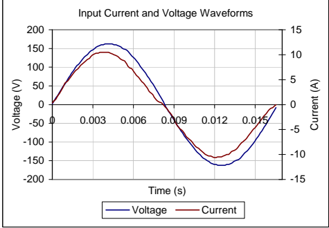
Input AC Current Waveform (ITHD = 9.83%, 50% Load)
