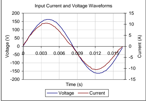
Input AC Current Waveform (ITHD = 6.93%, 50% Load)
