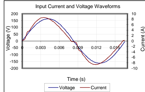
Input AC Current Waveform (ITHD = 12.91%, 50% Load)
