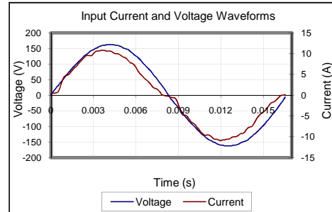
Input AC Current Waveform (ITHD = 15.94%, 50% Load)
