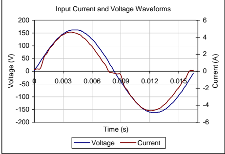
Input AC Current Waveform (ITHD = 13.31%, 50% Load)
