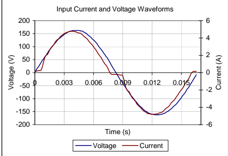
Input AC Current Waveform (ITHD = 12.69%, 50% Load)
