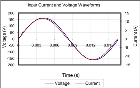
Input AC Current Waveform (ITHD = 6.9%, 50% Load)
