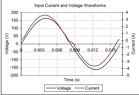
Input AC Current Waveform (ITHD = 10.41%, 50% Load)
