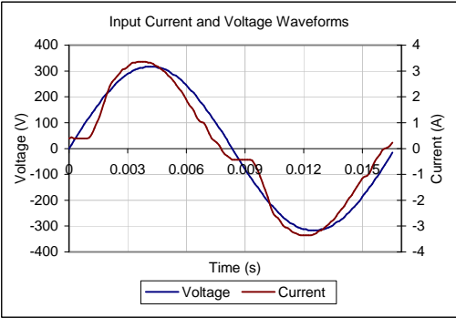
Input AC Current Waveform (ITHD = 18.2%, 100% Load)
