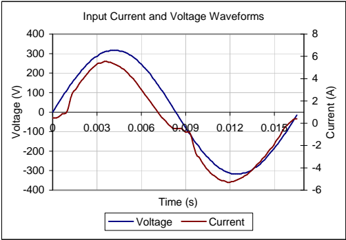
Input AC Current Waveform (ITHD = 14.48%, 100% Load)
