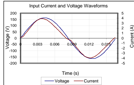
Input AC Current Waveform (ITHD = 10.87%, 50% Load)
