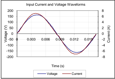
Input AC Current Waveform (ITHD = 6.78%, 50% Load)
