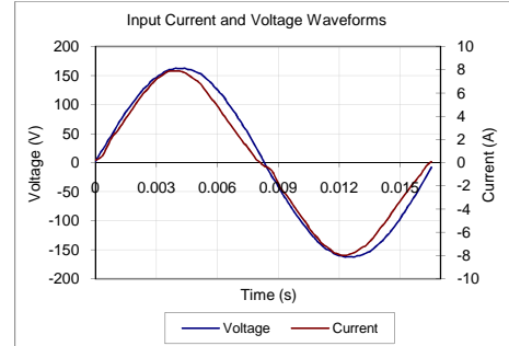
Input AC Current Waveform (ITHD = 10.77%, 50% Load)
