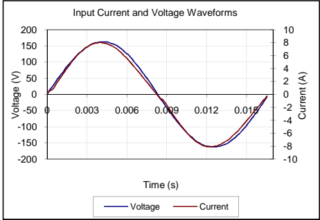
Input AC Current Waveform (ITHD = 6.24%, 50% Load)
