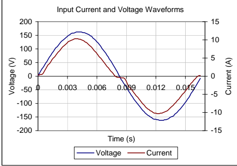
Input AC Current Waveform (ITHD = 17.55%, 50% Load)
