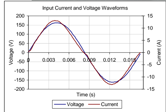
Input AC Current Waveform (ITHD = 11.07%, 50% Load)
