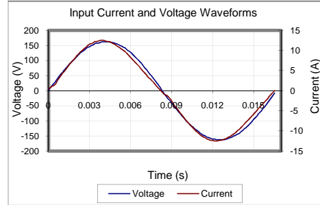
Input AC Current Waveform (ITHD = 7.73%, 50% Load)
