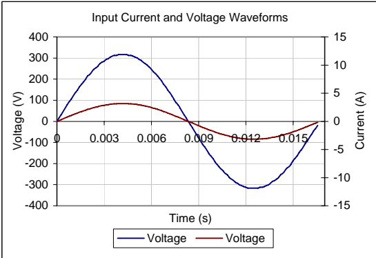
Input AC Current Waveform (ITHD = 20.02%, 100% Load)
