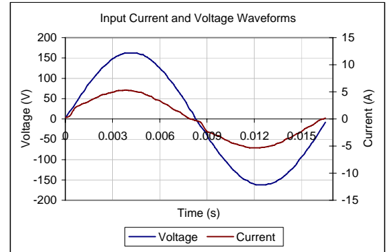
Input AC Current Waveform (ITHD = 9.01%, 50% Load)
