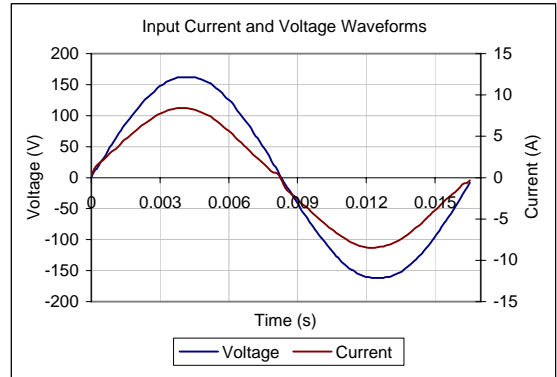
Input AC Current Waveform (ITHD = 3.42%, 50% Load)
