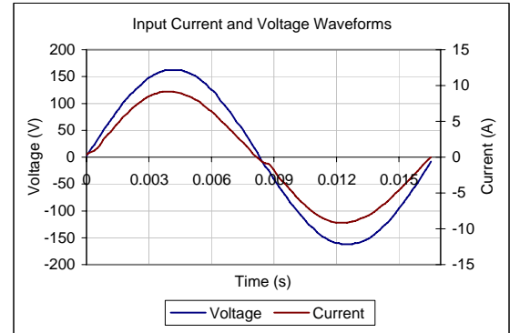
Input AC Current Waveform (ITHD = 4.49%, 50% Load)
