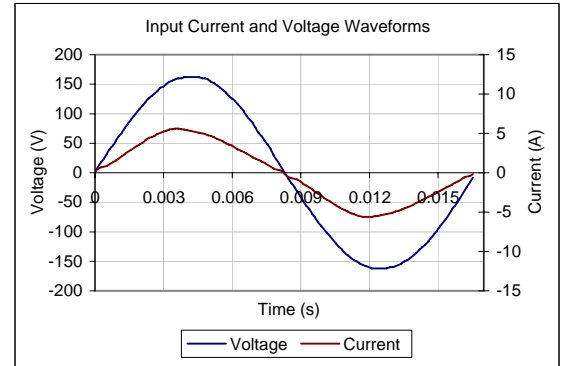
Input AC Current Waveform (ITHD = 13.07%, 50% Load)
