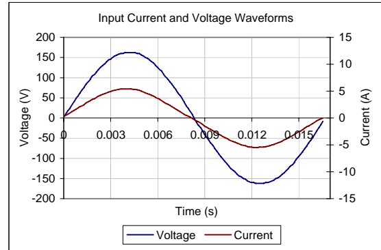
Input AC Current Waveform (ITHD = 5.76%, 50% Load)
