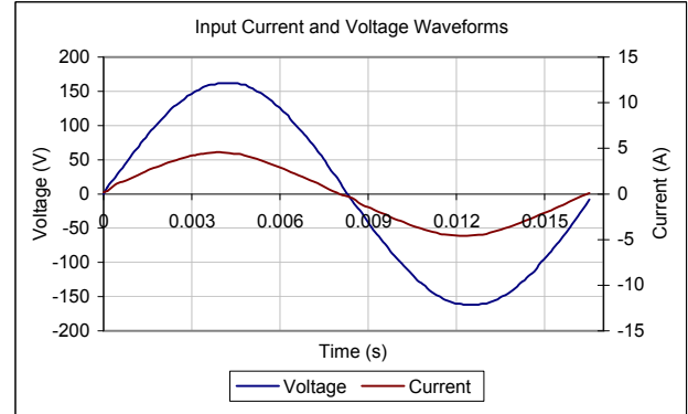
Input AC Current Waveform (ITHD = 5.5%, 50% Load)
