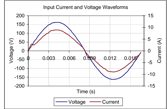
Input AC Current Waveform (ITHD = 3.31%, 50% Load)
