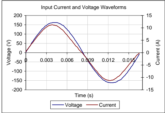
Input AC Current Waveform (ITHD = 6.74%, 50% Load)
