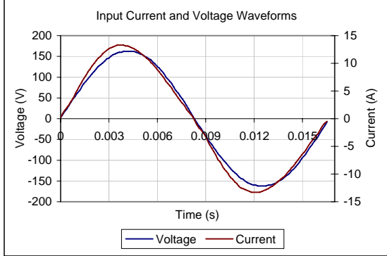
Input AC Current Waveform (ITHD = 3.53%, 50% Load)
