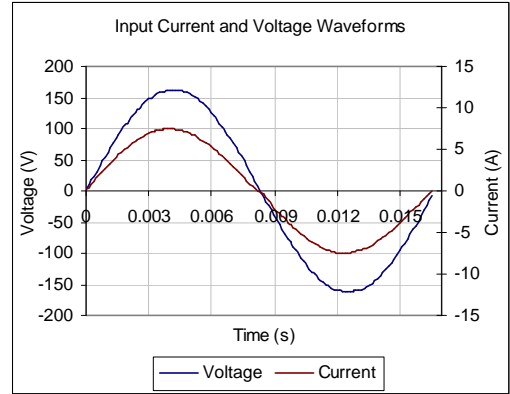
Input AC Current Waveform ( I_{THD} = 4.3\% , 50% Load)
