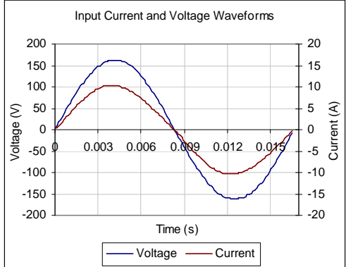
Input AC Current Waveform (ITHD = 4.39%, 50% Load)
