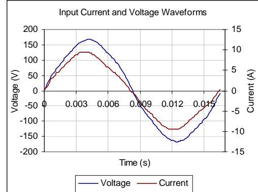
Input AC Current Waveform ( I_{THD} = 5.9\% , 100% Load)
