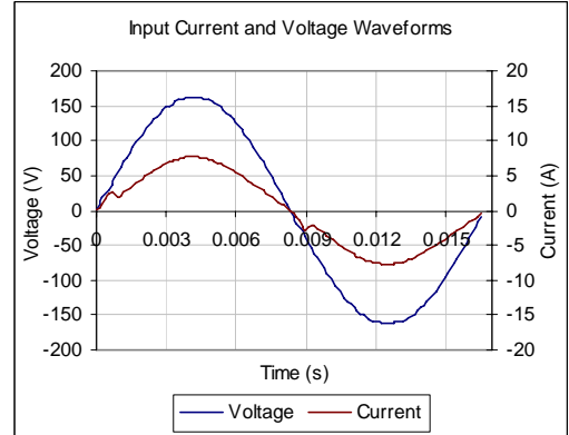
Input AC Current Waveform ( I_{THD} = 5.7\% , 50% Load)
